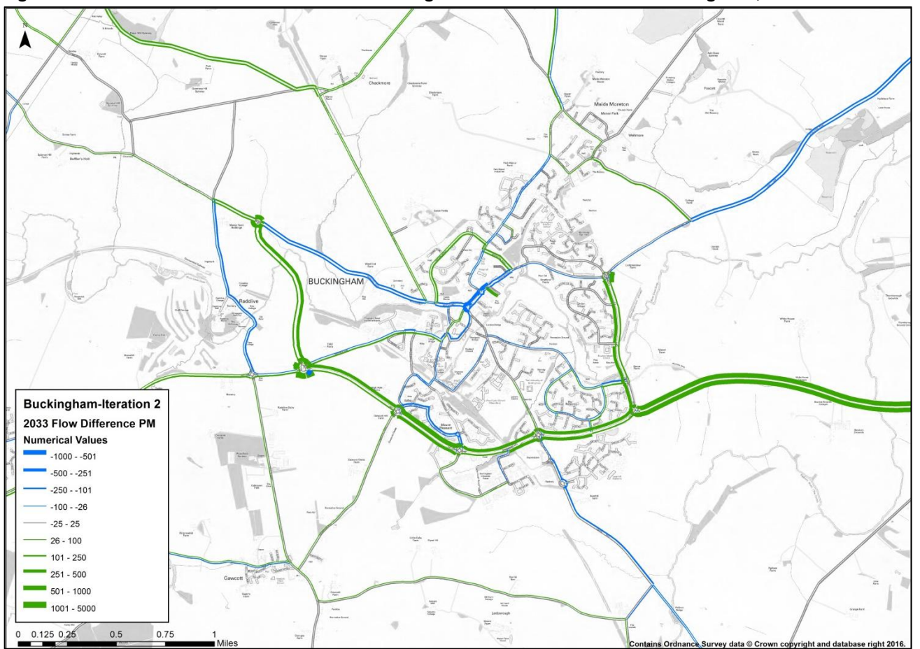
Figure 4.11: PM Peak Flow Difference – DS1 with mitigation minus 2033 DS1 without mitigation, 2033
