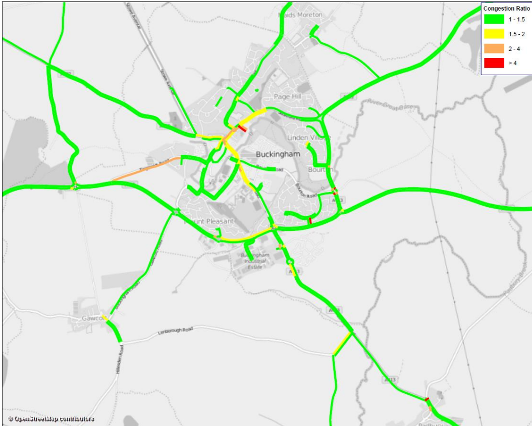
Figure 2.21: AM Peak Performance Plots in Buckingham, 2013 37
